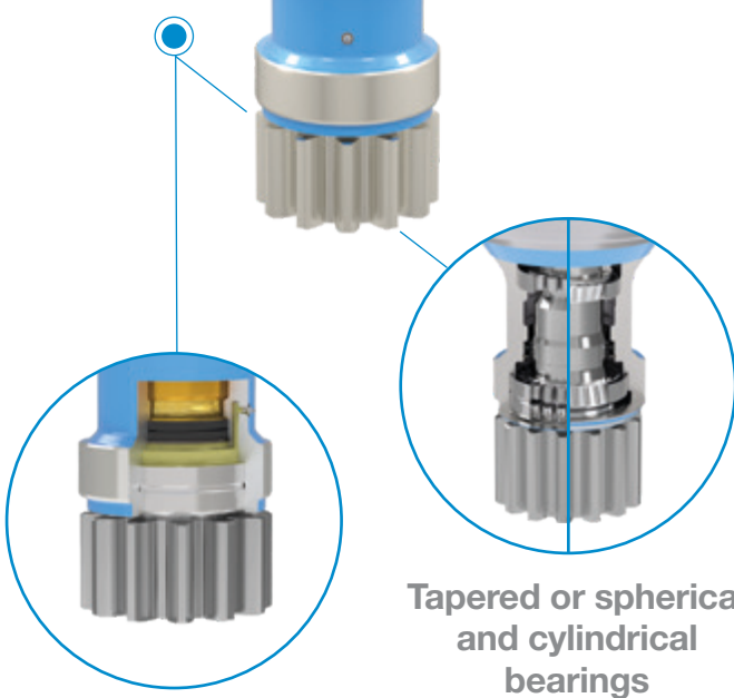
Grease lubrication outer bearing
